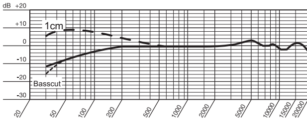
Frequenzgang (Hyperniere)
